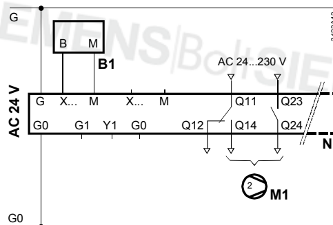
Connection diagram 5: 2-speed motor control (fan)
