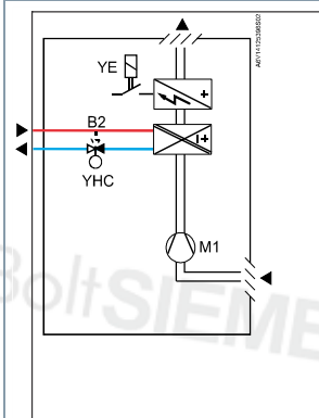
2-pipe fan coil unit with electric heater
