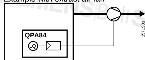
Example with extract air fan
