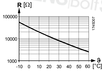
Characteristic curve:
