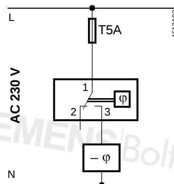
Diagram 2: Dehumidification
