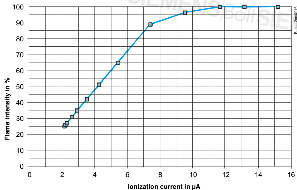
Ionization probe
