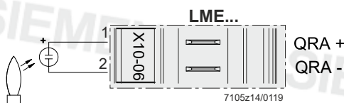
UV flame detector QRA
