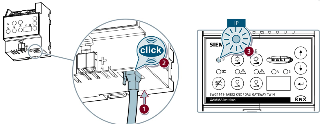
Fig. 9: KNX/DALI Gateway - Ethernet connection
