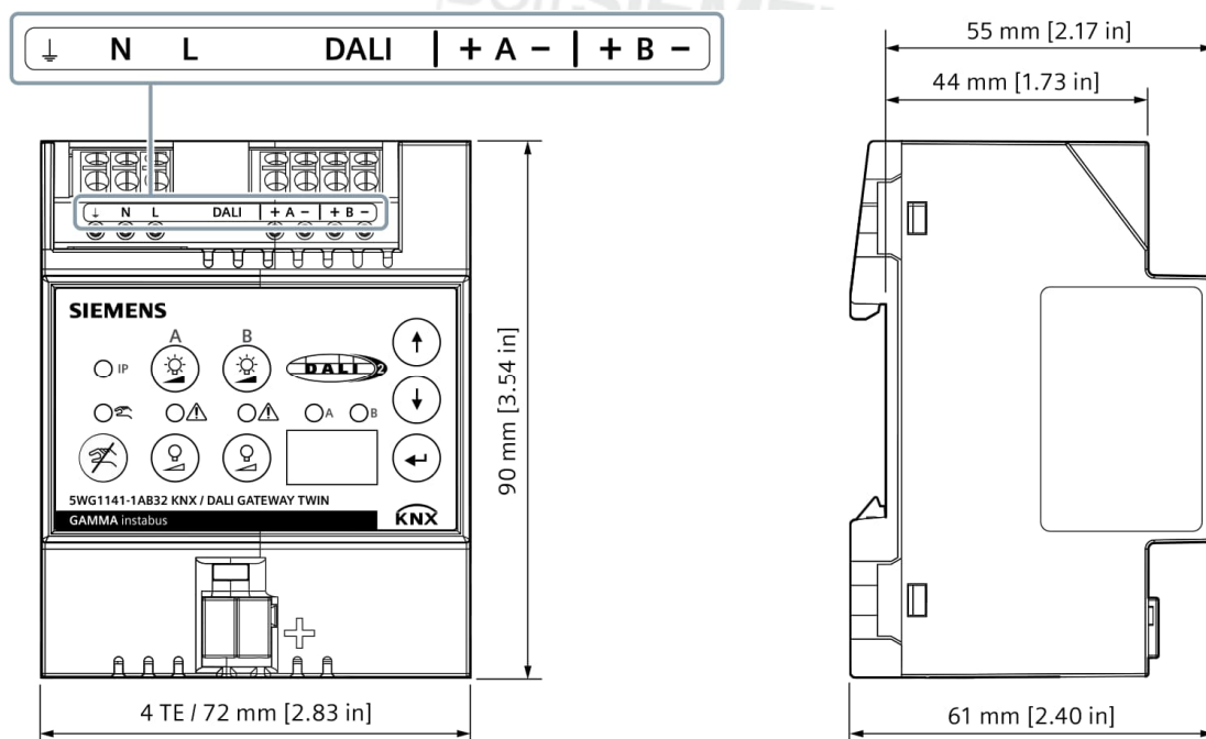
Fig. 13: KNX/DALI Gateway - dimensional drawing
