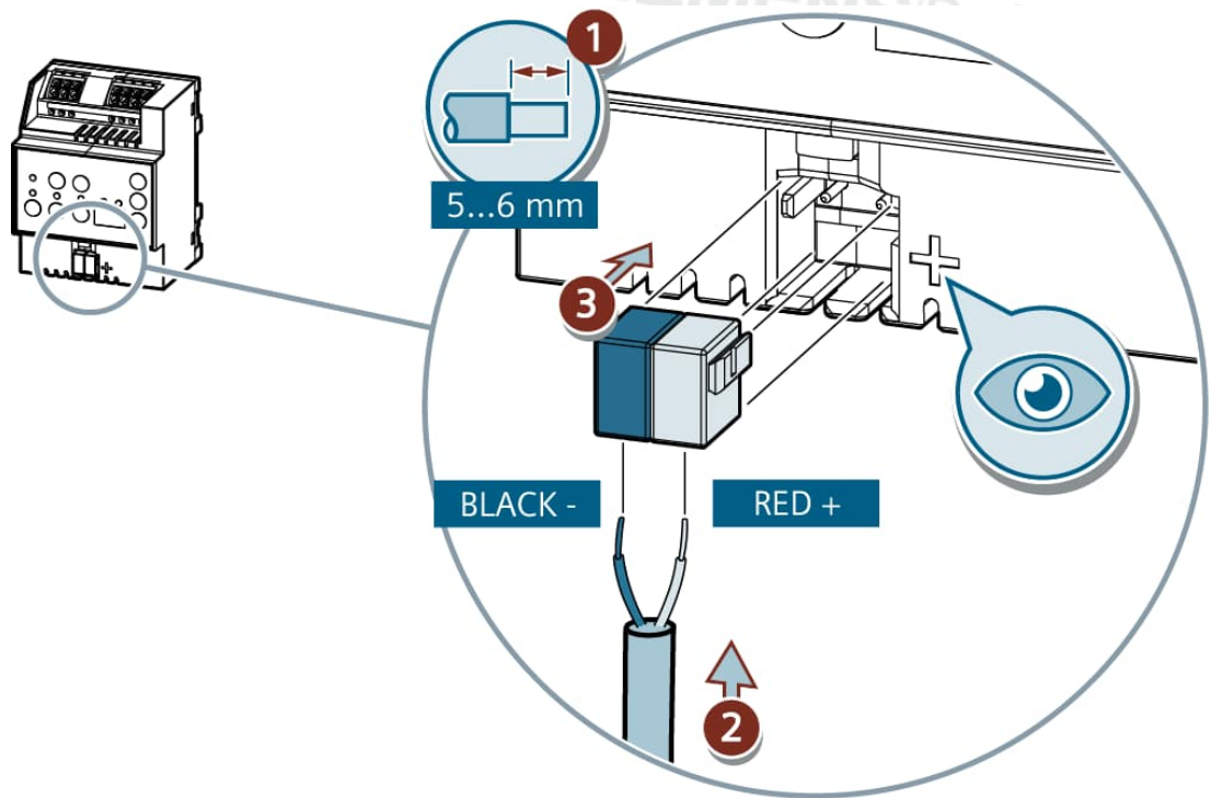
Fig. 8: KNX/DALI Gateway - connection of KNX
