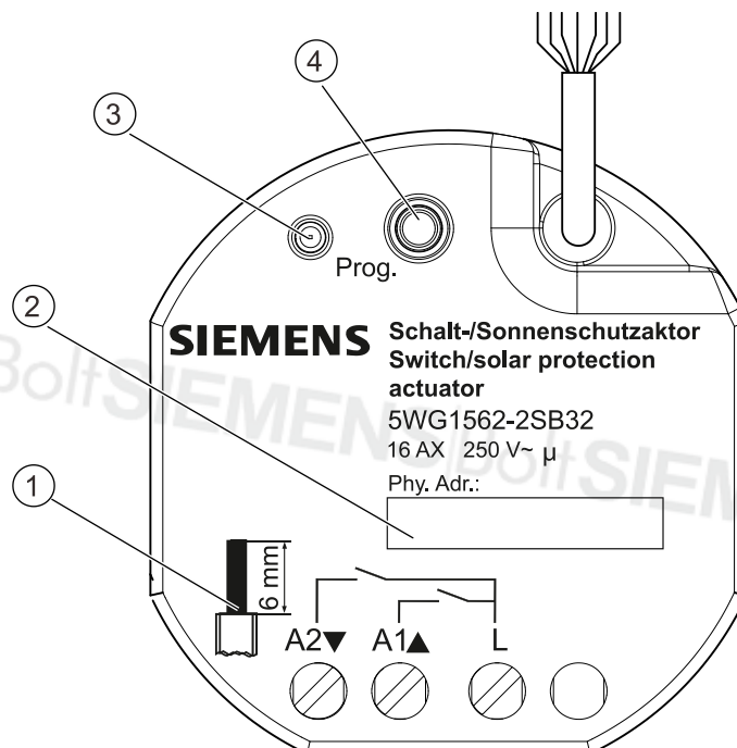
Fig. 2: Connections, operating and display elements
