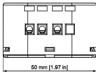
Fig. 8: Dimensions
